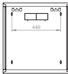
Rear view
