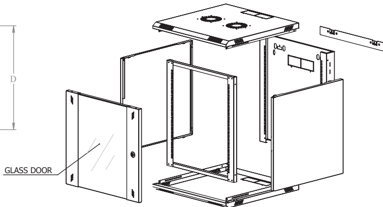
EXPLODED VIEW
