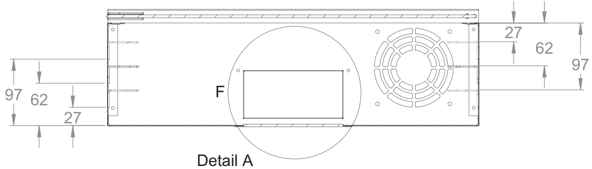
2U 19" mounting rails top view
