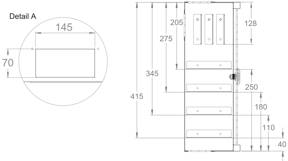
3U 19" mounting rails side view
