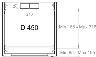
Max. / Min Equipment mounting distance (450)
