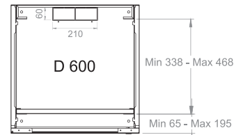
Max. / Min Equipment mounting distance (600)
